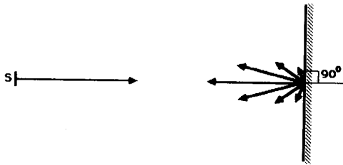
Fig. 2. Reflections of sound waves from smooth surface perpendicular to acoustic axis.
