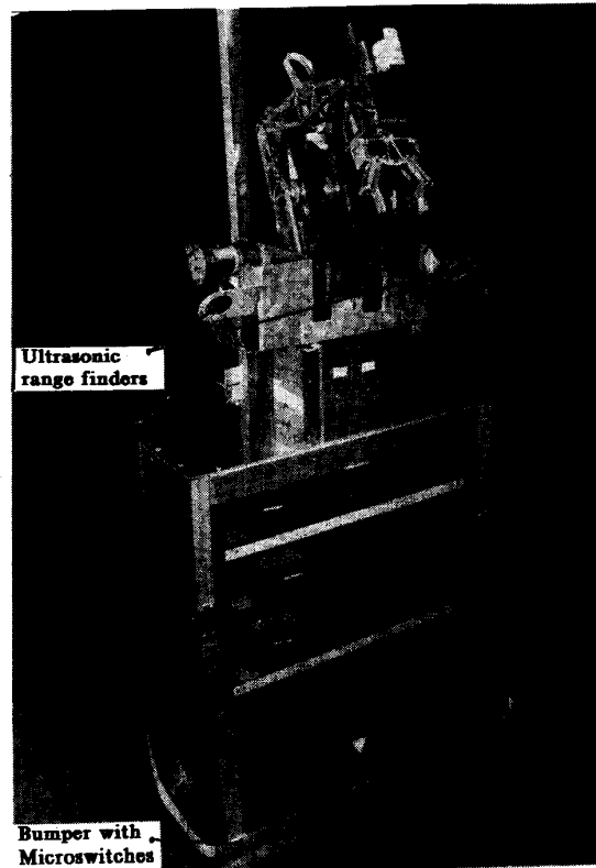
Fig. 1. Technion's nursing robot.
